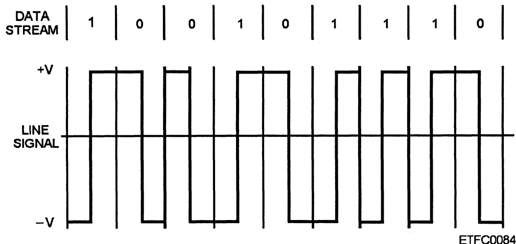
Figure 7-22.—Manchester code used in Ethernet
