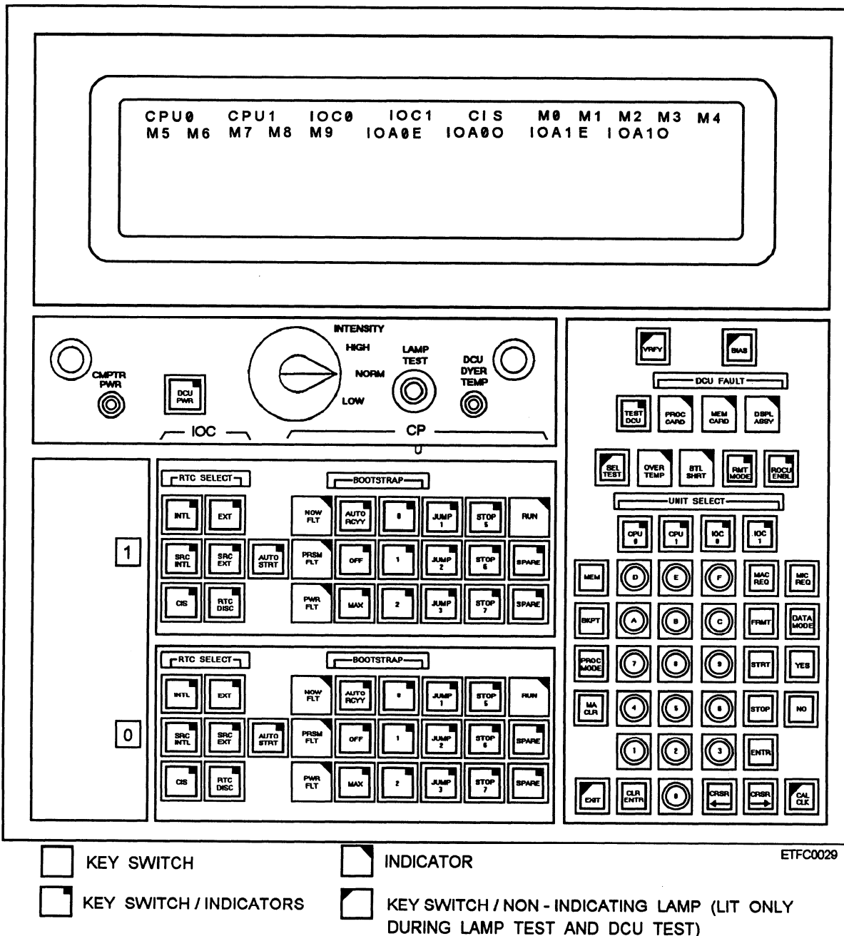
Figure 3-6.—Example of a display control unit (DCU).
