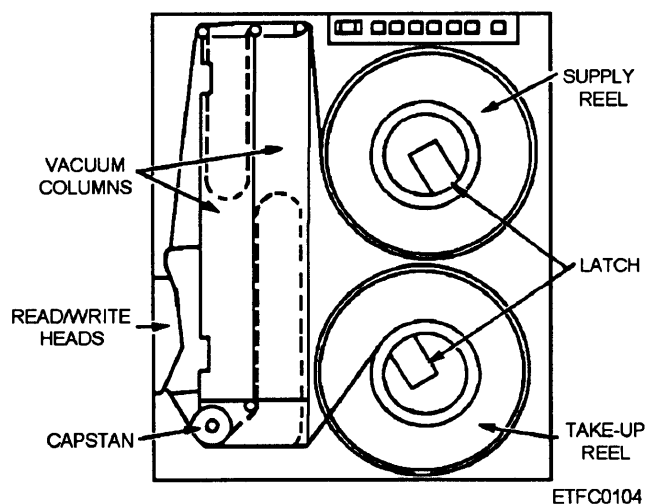
Figure 9-8.—A magnetic tape transport
