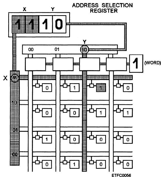
Figure 6-4.—Row (X), column (Y) organization.
