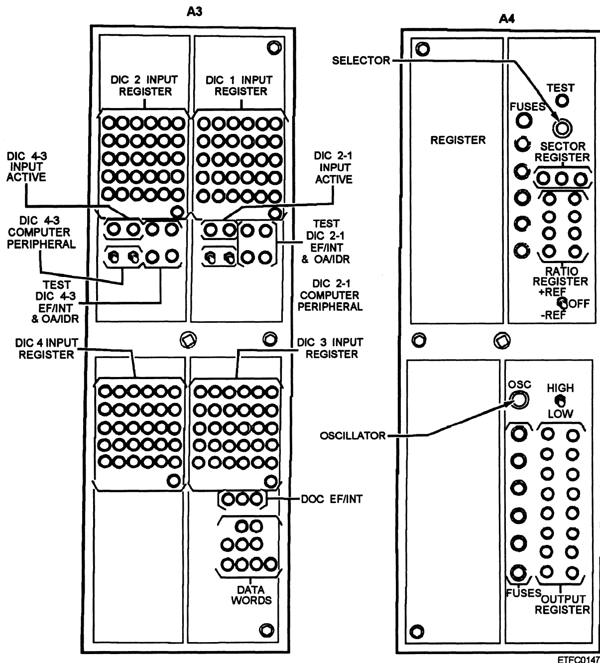
Figure 13-13.—KCMX front panels (A3/A4).
