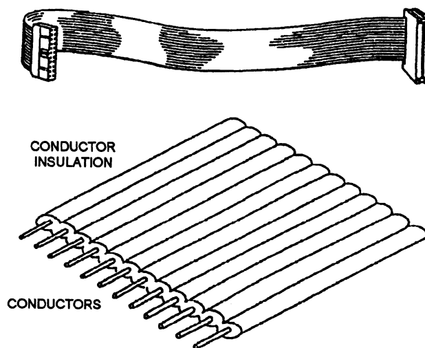
Figure 2-33.—Ribbon cable.
