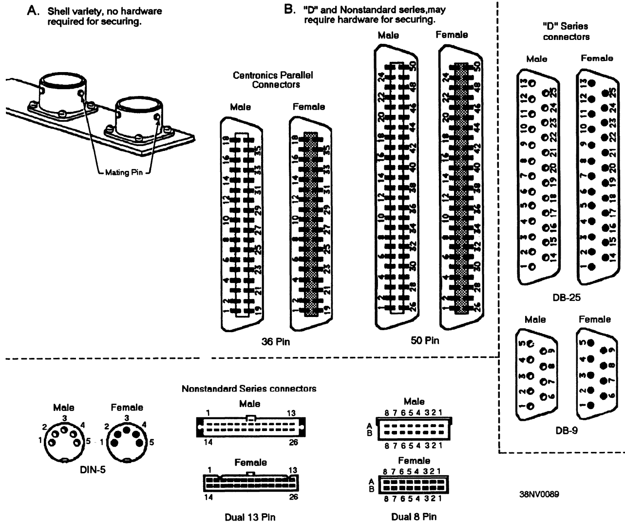
Figure 2-30.—Examples of the different types of external connector receptacles used by computers.
