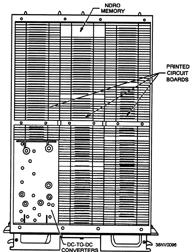
Figure 2-9.—Example of an individual physical layout of a module used in a mainframe computer.
