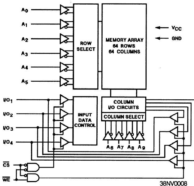
Figure 6-31.—Block diagram of a 1K × 4 SRAM.
