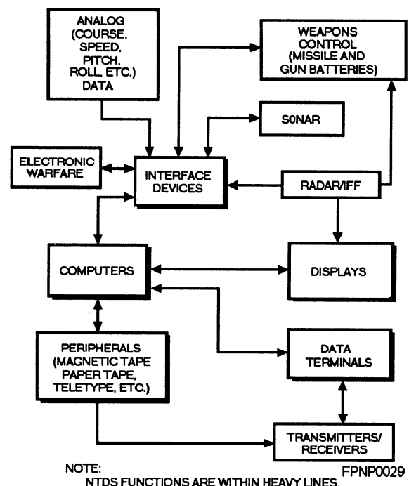
Figure 1-6.—Simplified block diagram of a tactical data system (CDS/NTDS).
