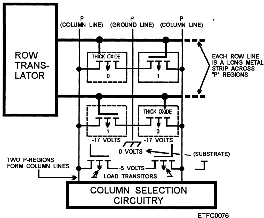
Figure 6-37.—MOS ROM.
