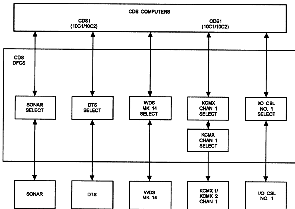
Figure 13-18.—Equipment interconnection through the CDS DFCS.
