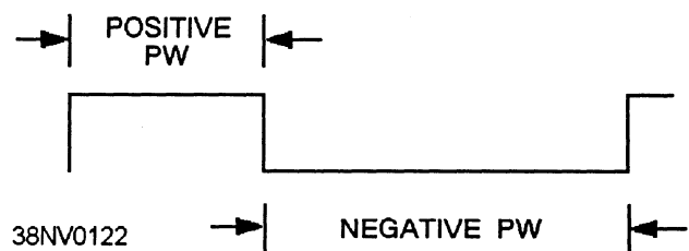
Figure 4-7.—Examples of pulse width (PW) measurements.
