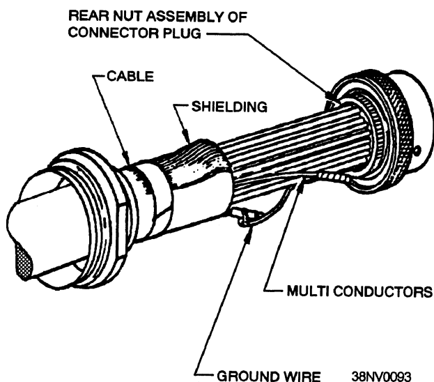
Figure 2-31.—Grounding a cable.
