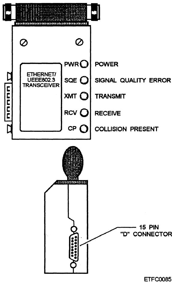
Figure 7-24.—Ethernet/IEEE 802.3 transceiver.
