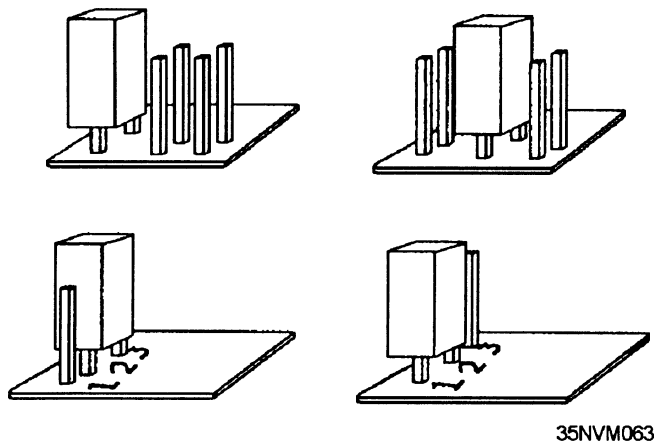
Figure 8-19.—Jumper connections.
