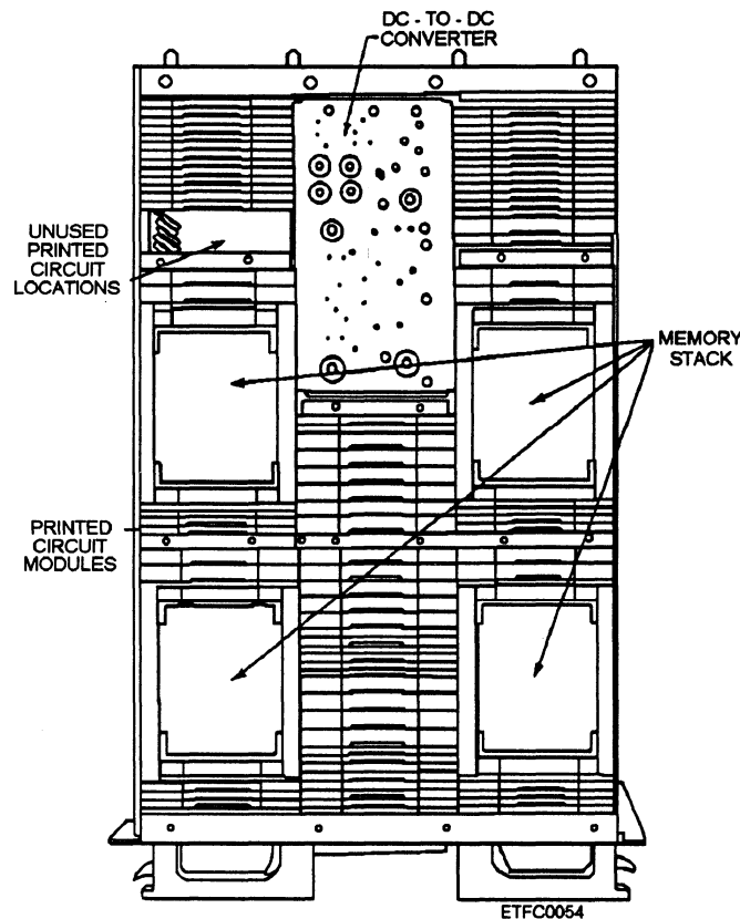
Figure 6-2.—Memory module/unit.
