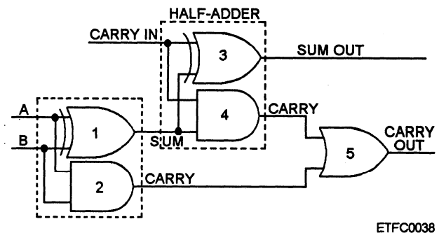
Figure 4-16.—Example of a full-adder circuit.
