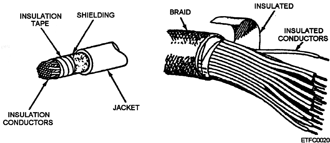
Figure 2-34.—Twisted component or multiconductor cable.
