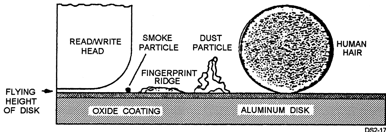
Figure 10-17.—The flying height of a disk read/write head compared to common contaminants.
