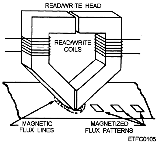
Figure 9-9.—Writing data on magnetic tape.
