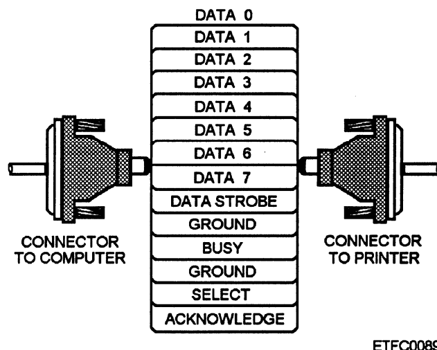
Figure 7-28.—Single parallel cable.
