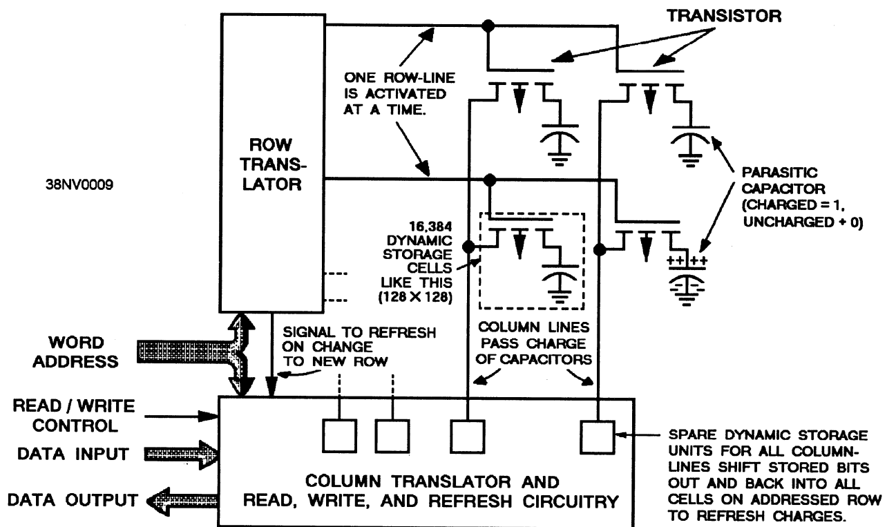
Figure 6-32.—DRAM storage cell.
