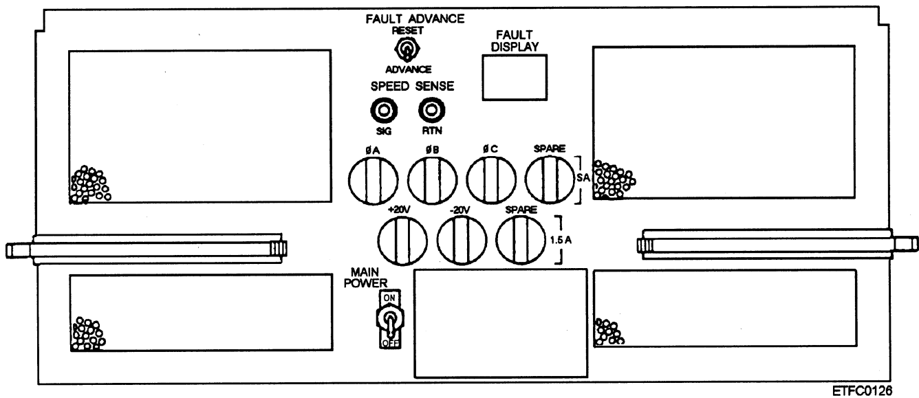
Figure 10-14.—A power supply panel.
