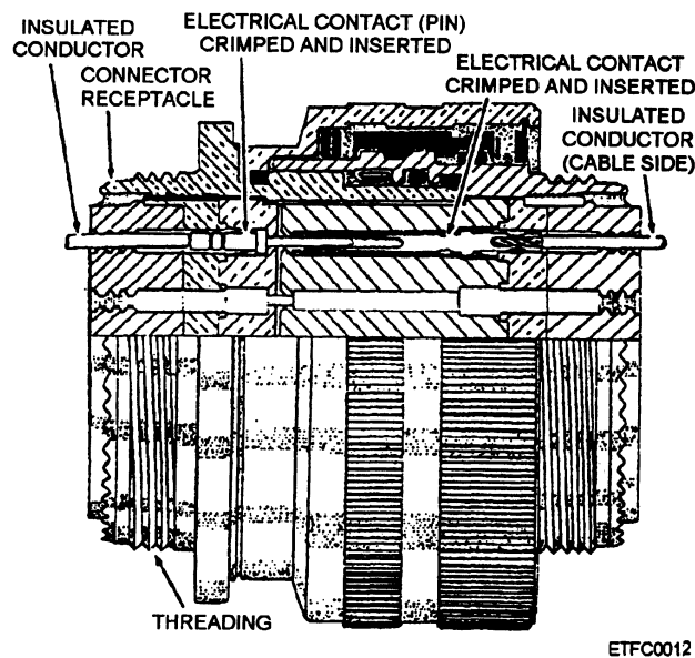
Figure 2-21.—Circular multipin connector.
