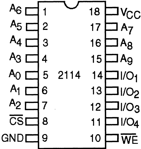
35NVM026 Figure 6-30.—SRAM IC chip with connections.
