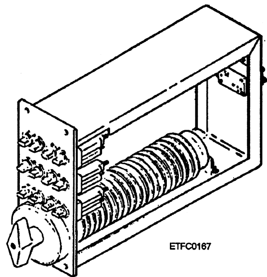
Figure 13-37.—Manually operated JR switch panel assembly.
