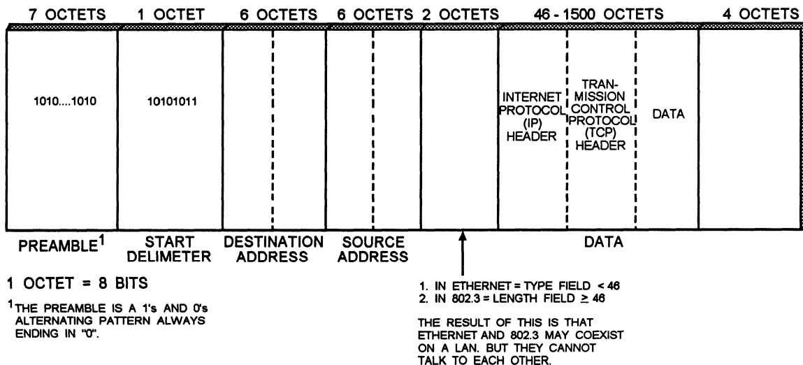
Figure 7-21.—802.3 and Ethernet packet formats.
