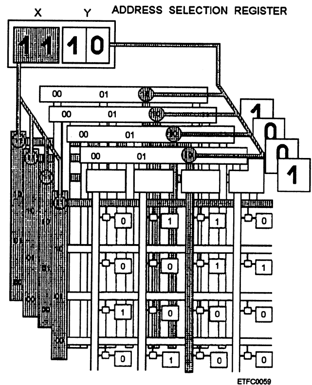
Figure 6-6.—4-bit address.
