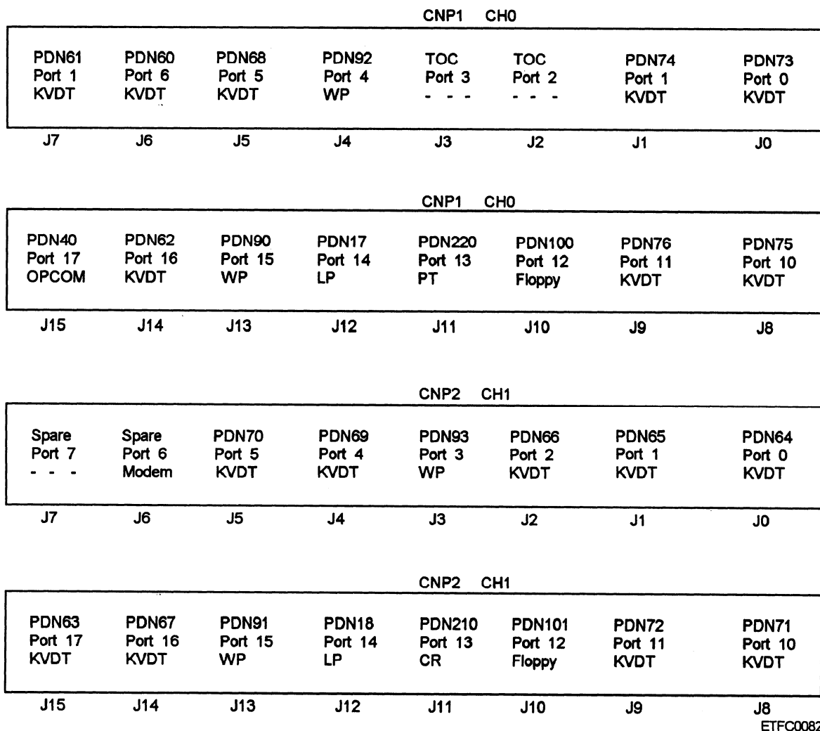
Figure 7-8.—Assigning multiple ports to a single channel.
