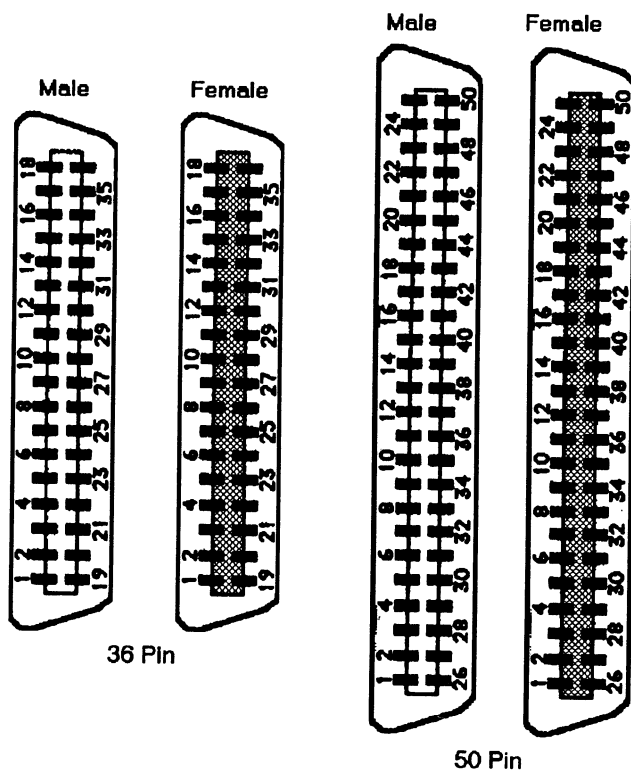
Figure 2-28.—Examples of connector receptacle physical shapes.
