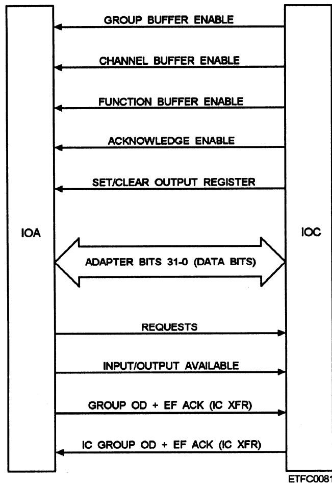
Figure 7-6.—IOA/IOC interface.
