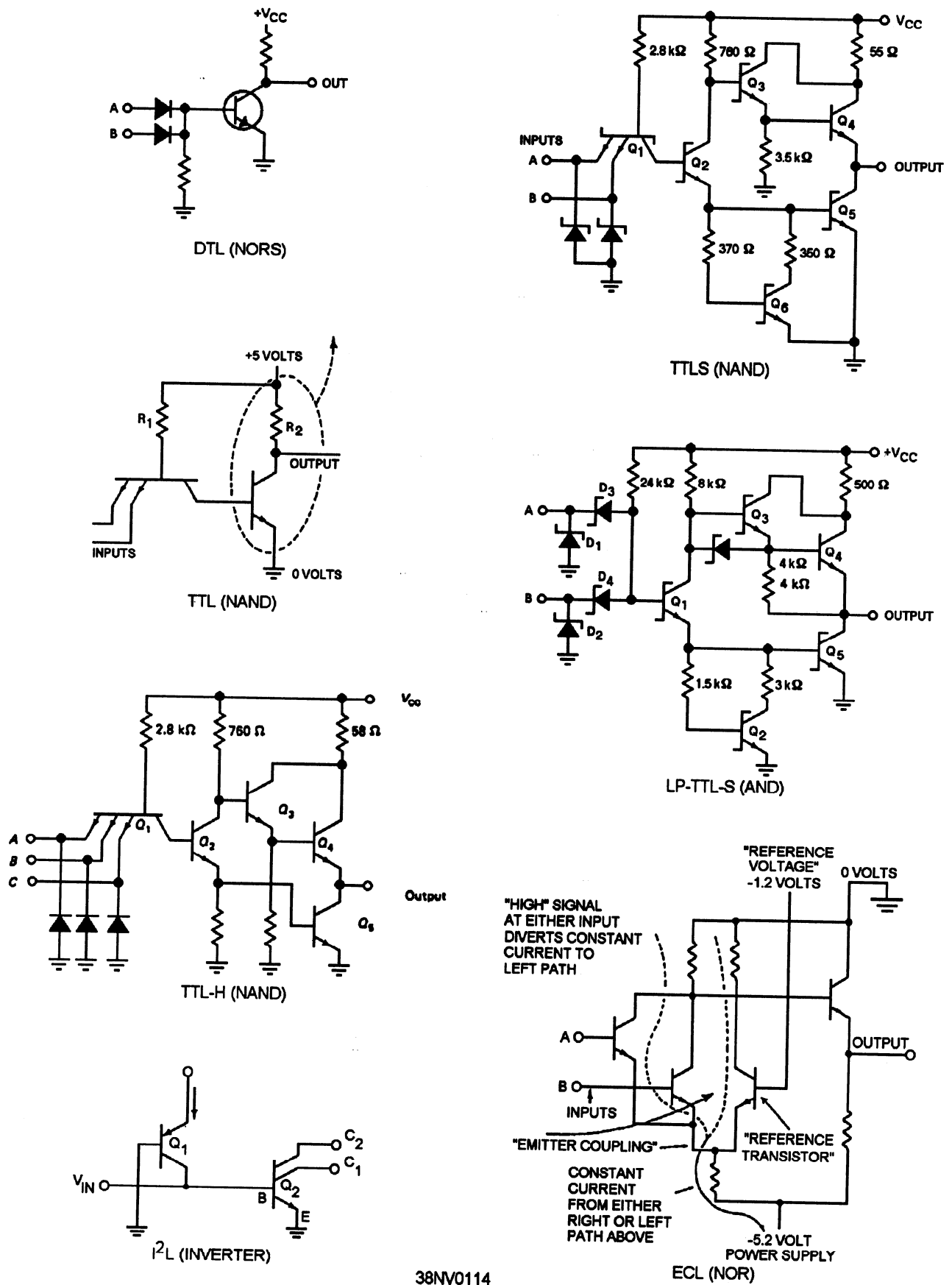
38NV0114 Figure 4-4.—Example schematics of bipolar ICs.
