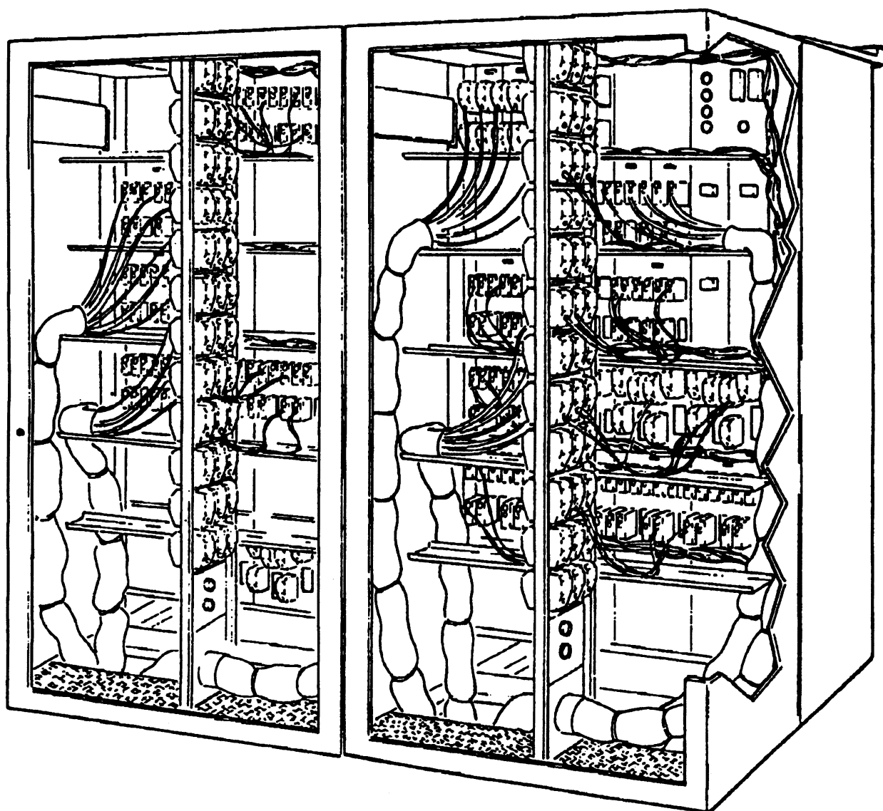
Figure 13-19.—DFCS interior.
