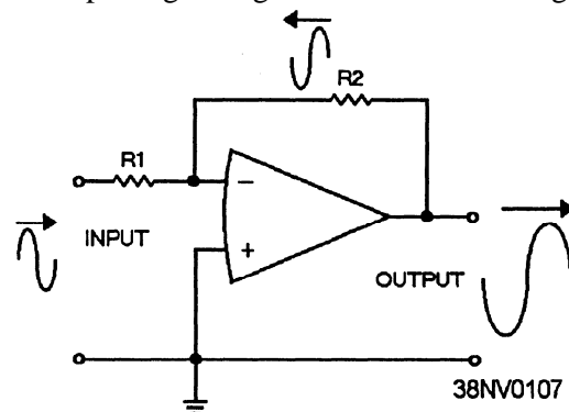
Figure 4-32.—Example of a closed-loop op amp.
