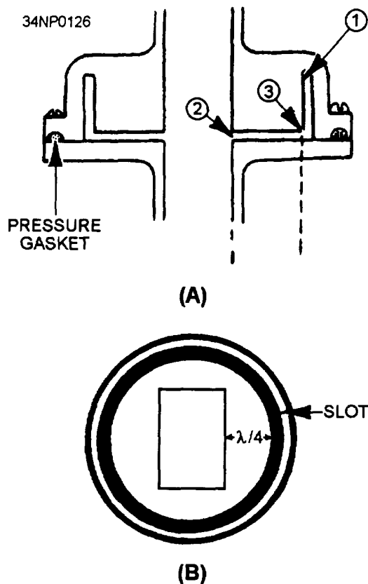
Figure 3-53.—Choke joint.
