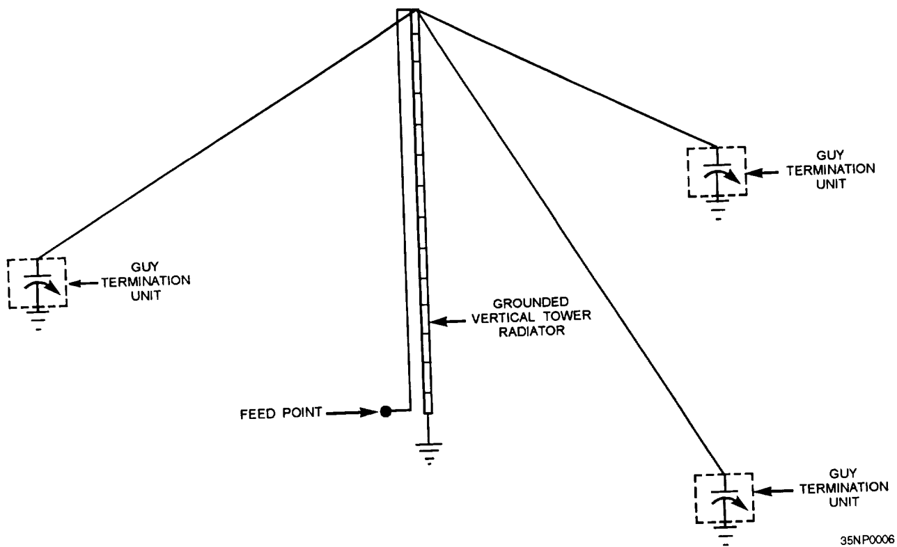
Figure 2-14.—NORD antenna.
