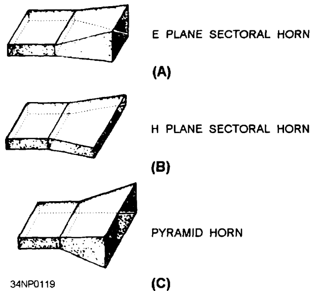
Figure 3-46.—Waveguide horns.
