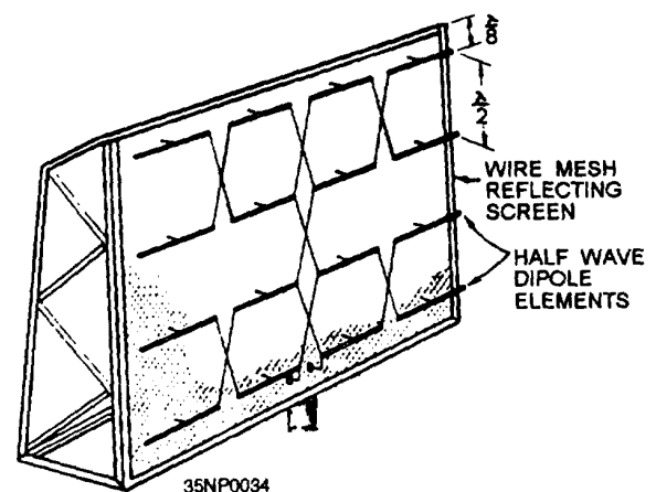
Figure 2-42.—Broadside array.
