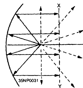
Figure 2-39.—Parabolic reflector radiation.
