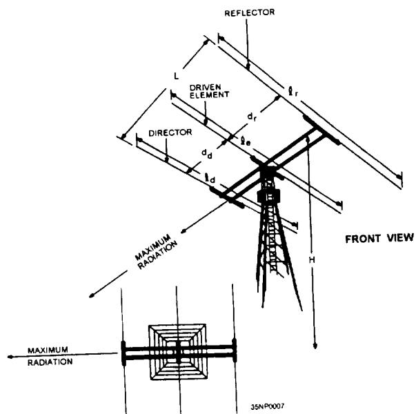
Figure 2-15.—Yagi antenna.
