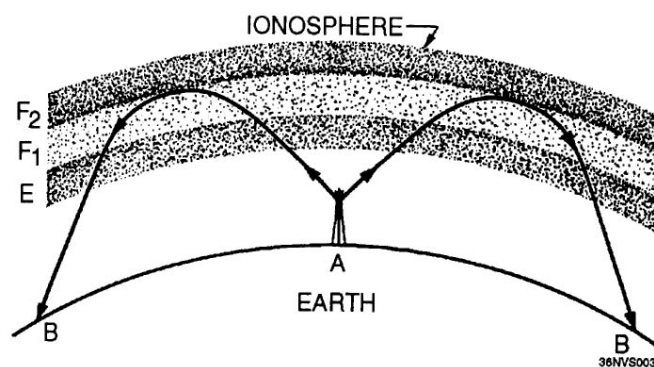
Figure 1-3.—Radio-wave refraction.
