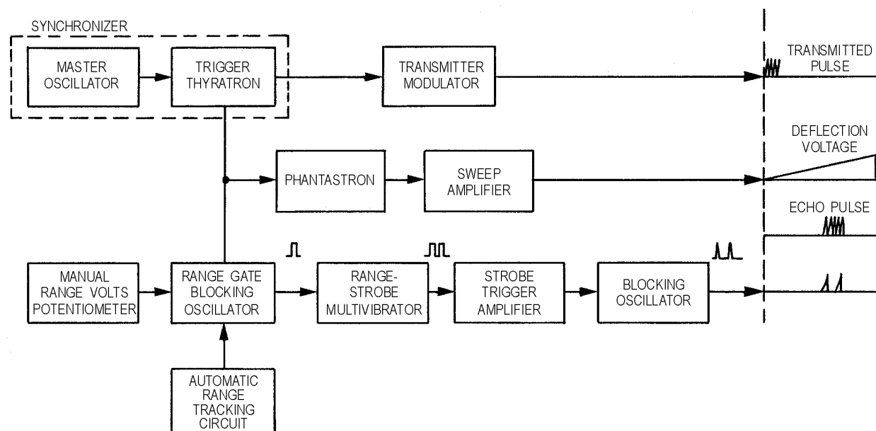
Figure 3-11.—Range-gate generator.
