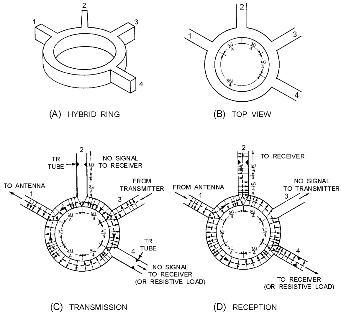
Figure 2-22.—Hybrid-ring duplexer.
