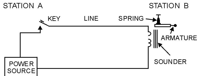
Figure 3-16.—Manual telegraph circuit.
