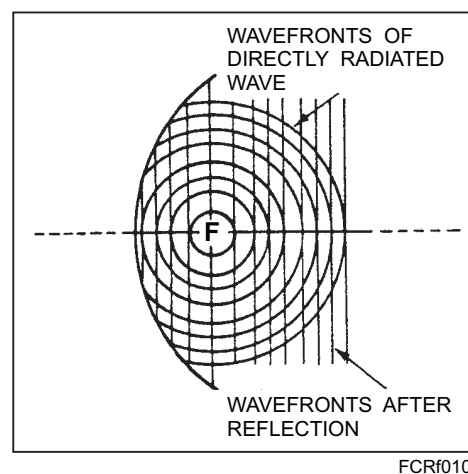
Figure 1-7.—Principles of the parabolic reflector.
