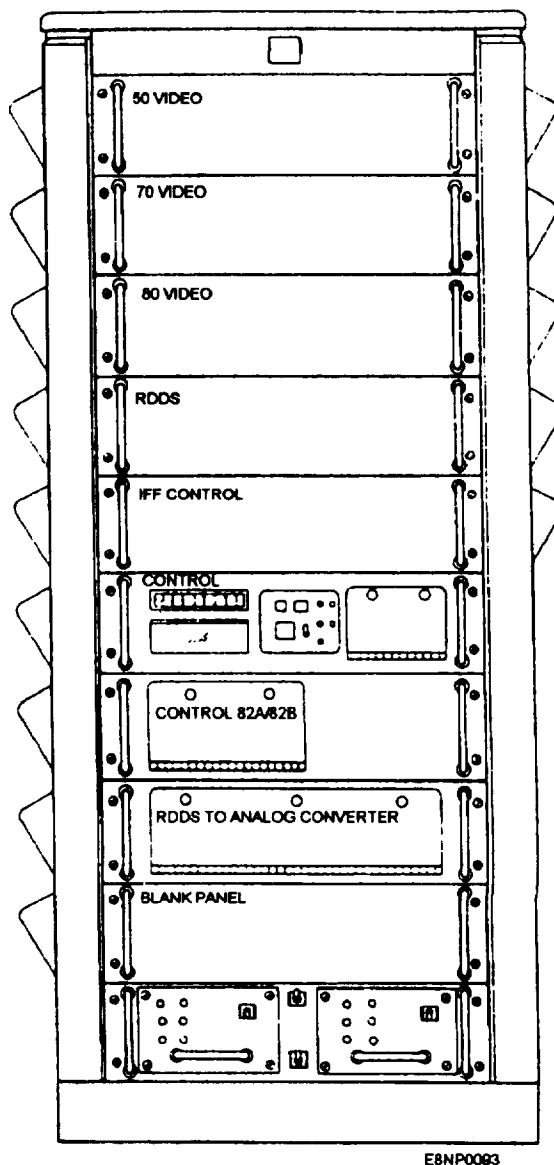
Figure 5-27.—Radar Distribution Switchboard, SB-4229/SP .
