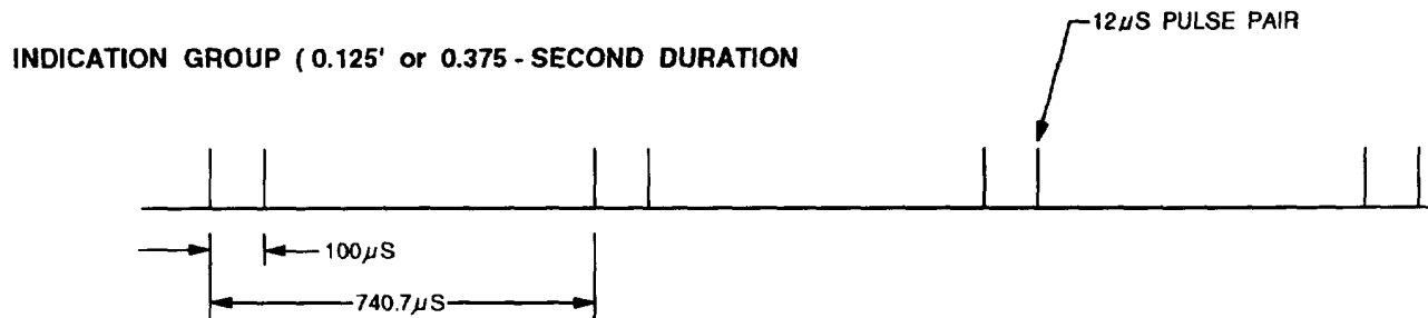
Figure 2-4.—Transponder output pulse train.
