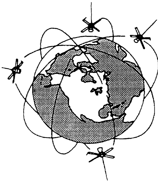
Figure 1-6.—Satellite orbits.
