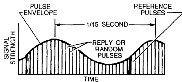
B. AMPLITUDE - MODULATED PULSE PAIRS
