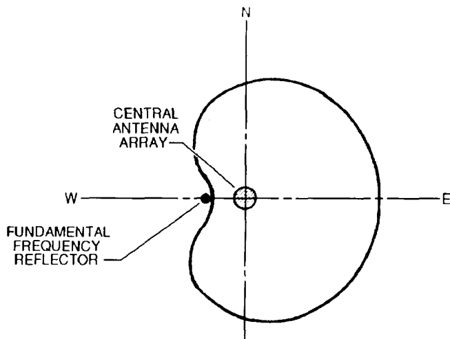
A. CARDIOID PATTERN
