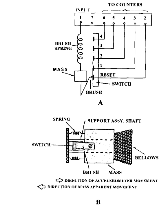
Figure 1-3.—Pulse counting accelerometer.
