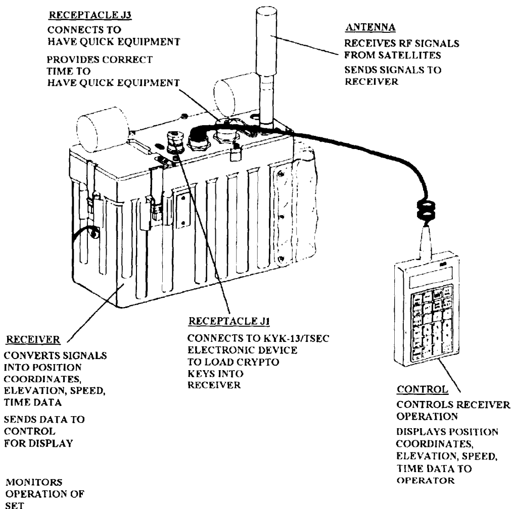
Figure 1-14.—Manpack Navigation Set AN/PSN-8( ).
