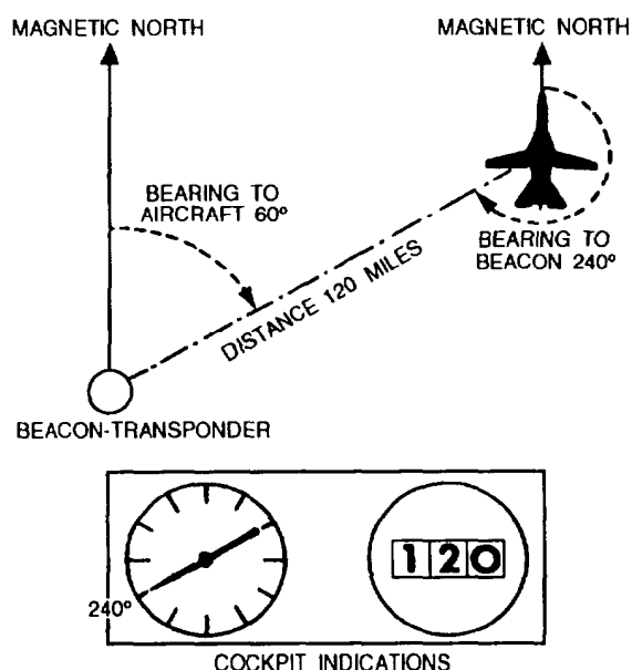
Figure 2-1.—TACAN aircraft indication.
